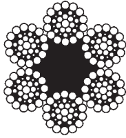
6x36 Warrington Seal with Fiber Core
